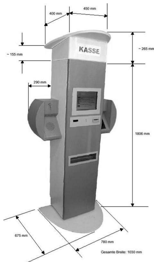
Medial Service-Terminal – Maße
